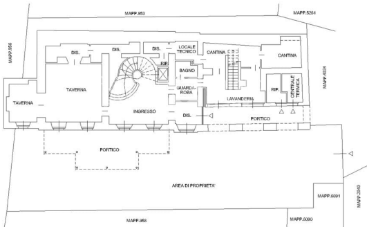
PIANO TERRA H: 2.80 m
