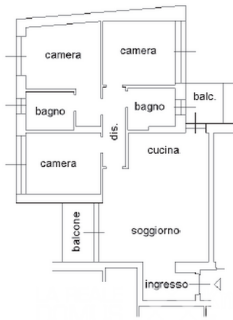
PIANO QUARTO H = 2,70 m
